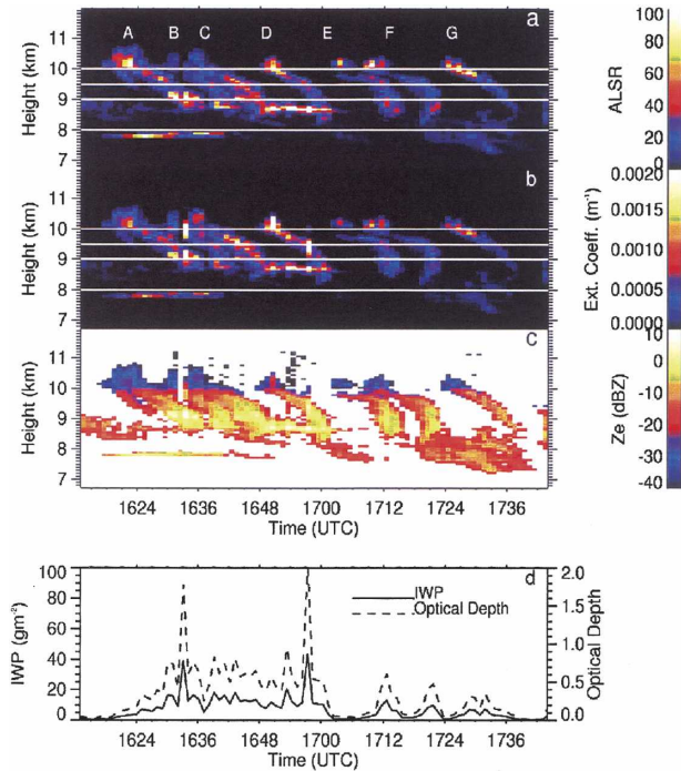
FIG. 6. The lidar observations taken at GSFC between 1612 and 1745 UTC for calculations of microphysical and radiative properties: (a) basic data, ALSR for fallstreaks A–G; (b) the extinction coefficient; (c) the estimated radar reflectivity factor computed from the data in (b); and (d) the corresponding IWP (left scale and solid curve) and optical depth ( \tau ) (right scale and dashed curve).
